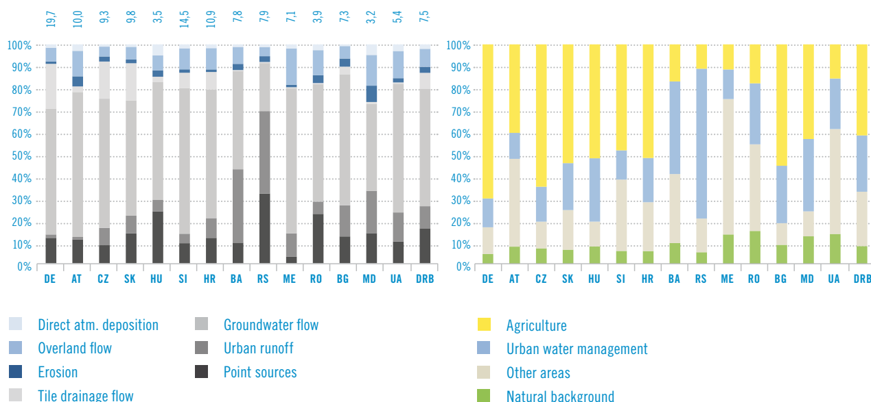
Share of the pathways and sources in the overall TN emissions in the Danube countries for the reference period (2009–2012); on the left: pathways, on the right: sources (absolute numbers on the top refer to kg N per hectare and year)
