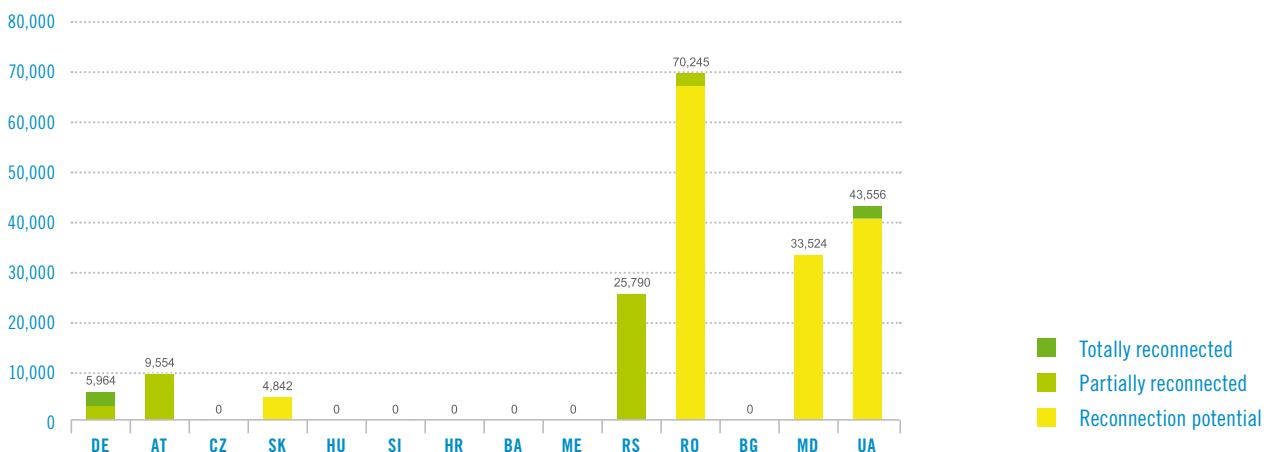
Area [ha] of DRBD wetlands/floodplains (> 500 ha or of basin-wide importance) which are reconnected or with reconnection potential
